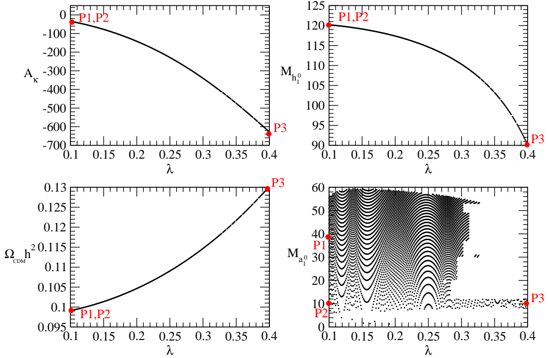
Figure 1: Allowed values of A_\kappa , M_{h_1^0} and M_{a_1^0} (in GeV) as well as \Omega_{\text{CDM}}h^2 as a function of \lambda . We take m_0 = 174 \text{ GeV} , M_{1/2} = 500 \text{ GeV} , A_0 = -1500 \text{ GeV} and \tan\beta = 10 ; m_{\tilde{g}}^2 is determined from the electroweak symmetry breaking conditions.
