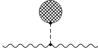
Figure 2. Tadpole diagrams which do not contribute to \Delta\rho .
