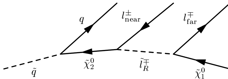
Figure 3: “Sequential” decay.
